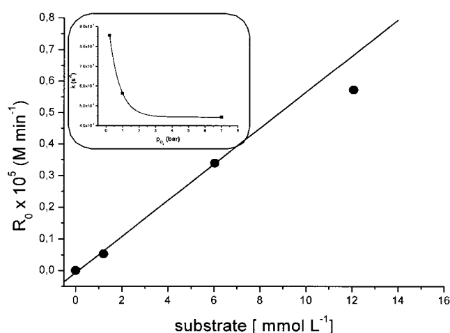
Figure 3. Kinetic order in substrate and oxygen (insert) for benzyl alcohol oxidation with \text{O}_2 catalysed by TP-Me3A (content of TPAP: 0.5 \times 10^{-2} mmol per 100 mg of ormosil), in \text{scCO}_2 at 22 MPa and 75 °C.
