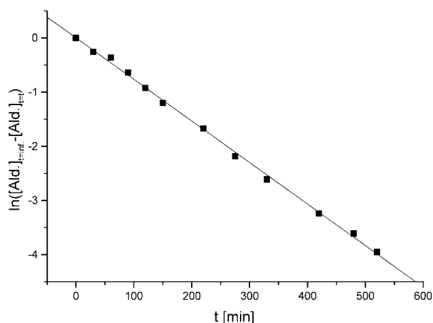
Figure 1. Plot of \ln([aldehyde]_{t=\infty} - [aldehyde]_{t=t}) vs. time in the oxidation of benzyl alcohol ( 4.83 \times 10^{-2} mmol) with oxygen (1 bar at 25 °C) catalysed by 20 mg of TP-Me3A (TPAP content of 1.0 \times 10^{-3} mmol) in scCO 2 at 22 MPa and 75 °C.
